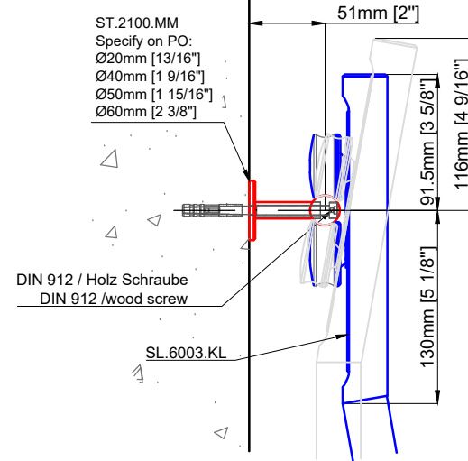
Detail Z
