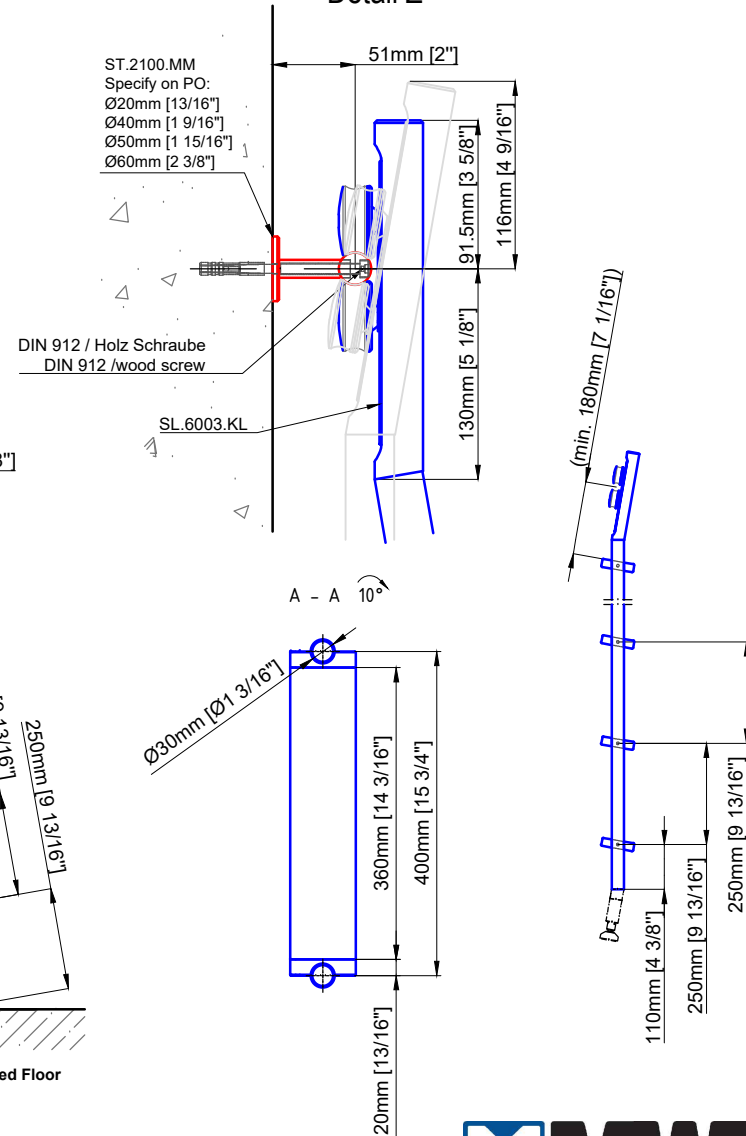
Detail Z
